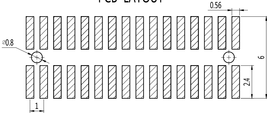
PCB LAYOUT
